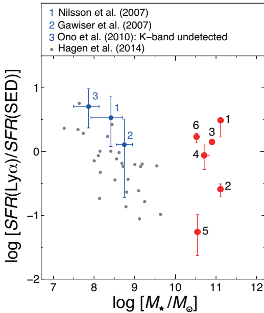
Figure 2. SFR(\text{Ly}\alpha)/SFR(\text{SED}) vs. M_* for our MAESTLOs (filled red circles) and LAEs at z \sim 3 from the literatures (filled blue circles for the results from stacked LAEs and filled gray circles for those from individual LAE). For Hagen et al. (2014), we plot only the LAEs at z = 2.5\text{--}3.2 in their sample. Note that the SFRs in the literatures derived with the Salpeter IMF are converted into those with the Chabrier IMF we use. Note also that Hagen et al. (2014) used the SFRs estimated from the dust-corrected UV luminosity instead of those based on the SED fitting.
