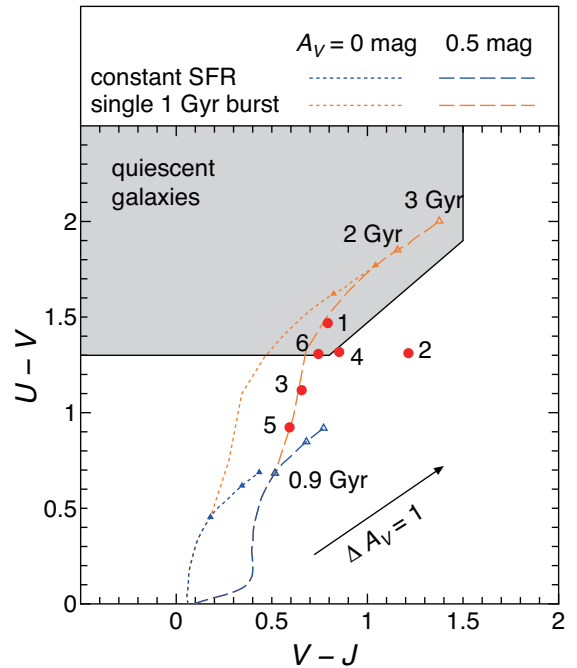
Figure 4. Rest-frame U - V vs. V - J two-color diagram for the MAESTLOs. The 6 MAESTLOs are shown by filled circles with their ID numbers. The domain of quiescent galaxies studied by Muzzin et al. (2013) is shown with the gray shaded area. Two star formation models (the constant star formation and the single 1 Gyr starburst) are also shown by blue and orange dotted curves for A_V = 0 and by blue and orange dashed curves for A_V = 0.5 mag.
