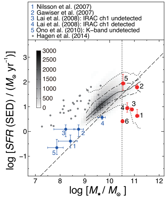
Figure 3. SFR(\text{SED}) vs. M_* for the same samples as shown in Figure 2 and for the LAE samples at z \sim 3.1 detected and undetected in IRAC 3.6 \mu\text{m} band. Our MAESTLOs are shown as filled red circles and LAEs from the literatures are shown as filled blue circles in the same manner as that in Figure 2. Note that SFR(\text{SED}) and M_* in the literatures derived with the Salpeter IMF are converted into those with the Chabrier IMF we use. We plot the so-called main sequence of star-forming galaxies at z_{\text{phot}} = 2.5\text{--}3.2 in the COSMOS field in gray scale with bin size of 0.1 dex in M_* and SFR. The scale (the number of galaxies per bin) is shown in the upper-left inset. Solid, dot-dashed, and dotted lines show the median, 16 and 84 percentiles, and 2.5 and 97.5 percentiles in bins of 0.1 dex in stellar mass. The dashed line shows the relation of sSFR = 1 \text{ Gyr}^{-1} . The vertical dotted line corresponds to \log (M_*/M_\odot) = 10.5 , which is one of the criteria of MAESTLO.
